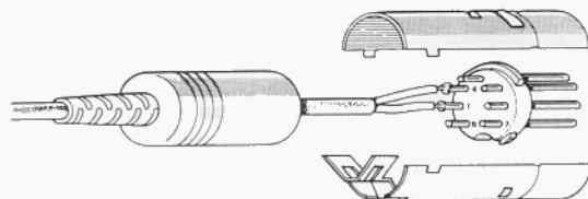
Fig. 5-1 Remote Terminal
