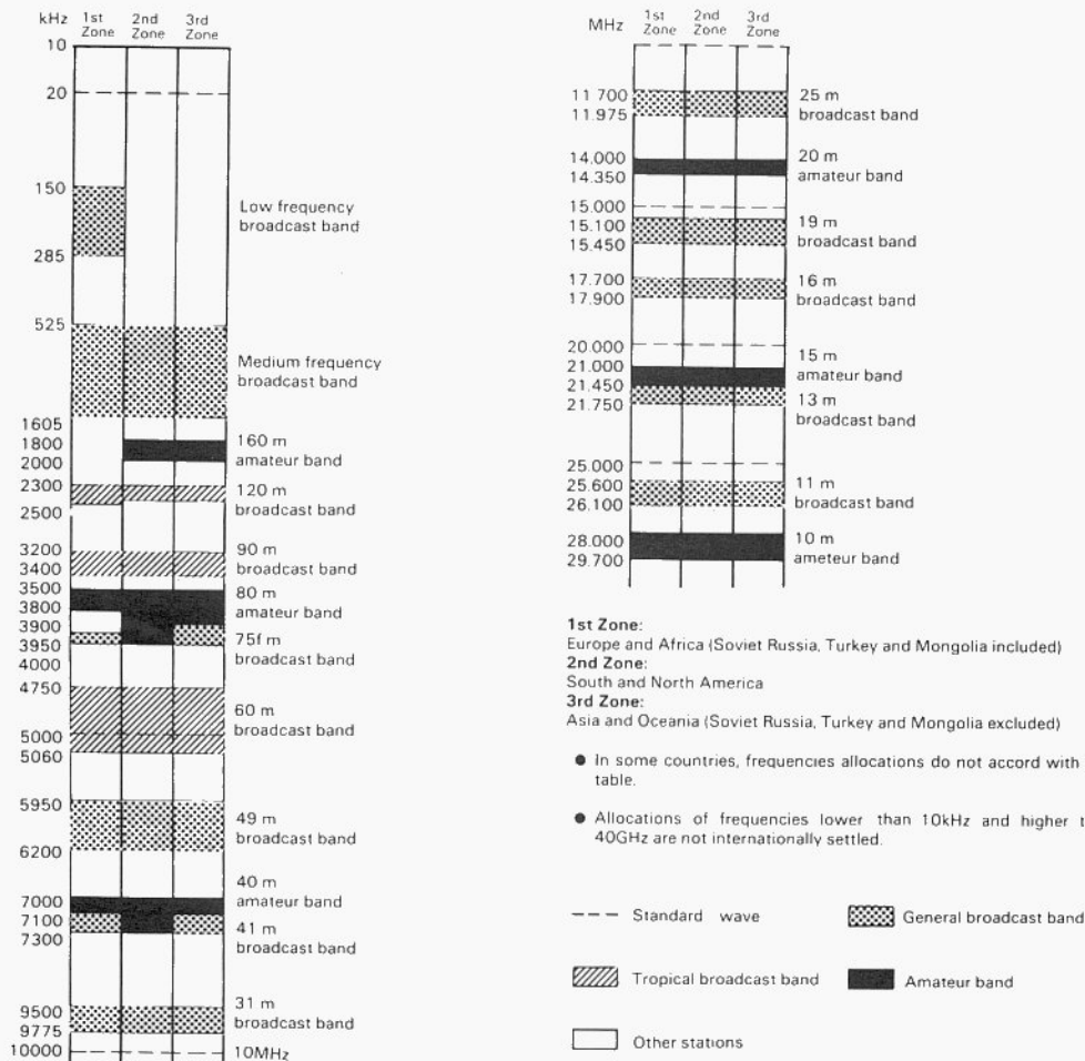
Fig. 6-2 Radio Frequency Allocation
