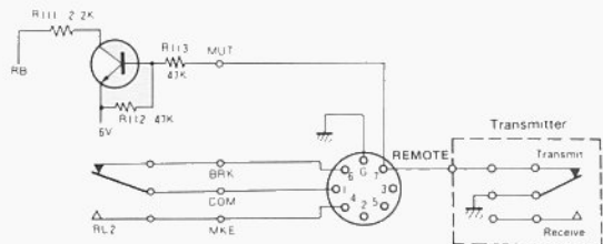
Fig. 5-1 Remote Terminal
